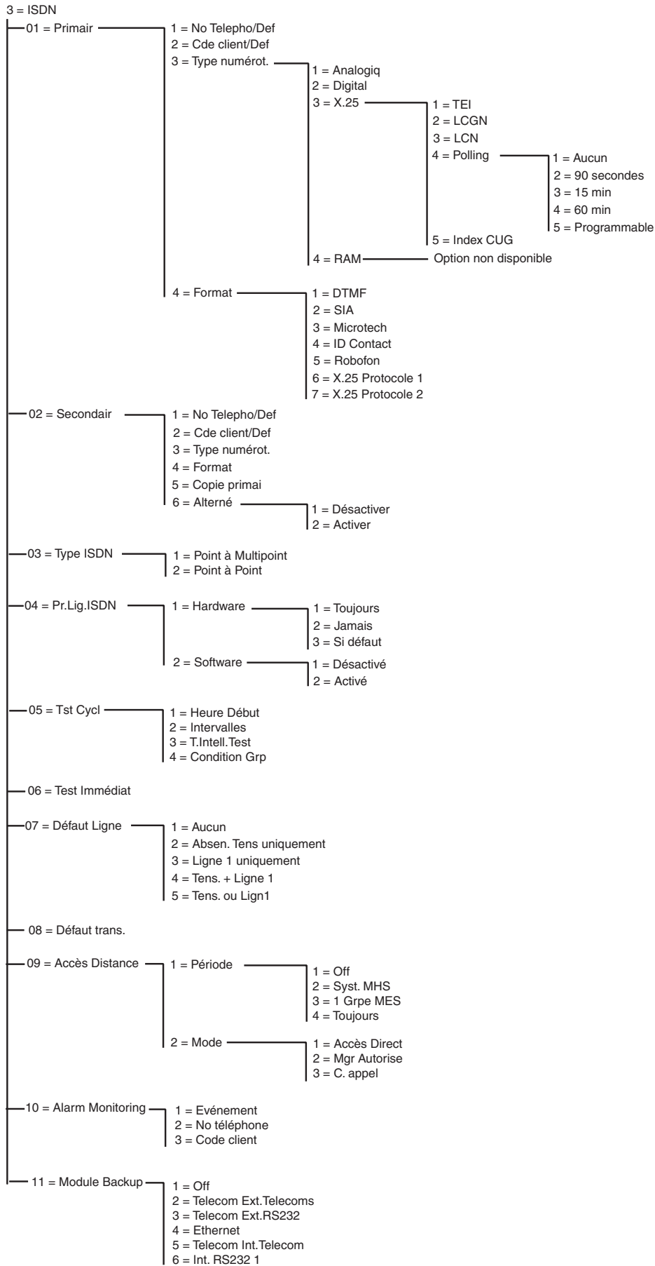
Figure 6-8. Structure de programmation ISDN
