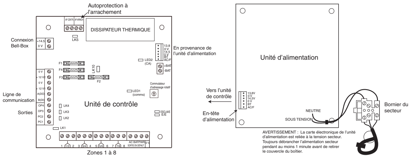
Figure 3-2. Alimentation PSU Galaxy
