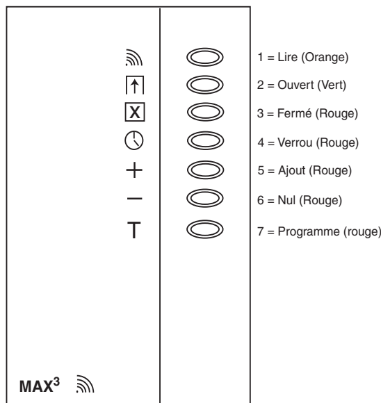
Figure 5-3. VOYANT MAX 3
